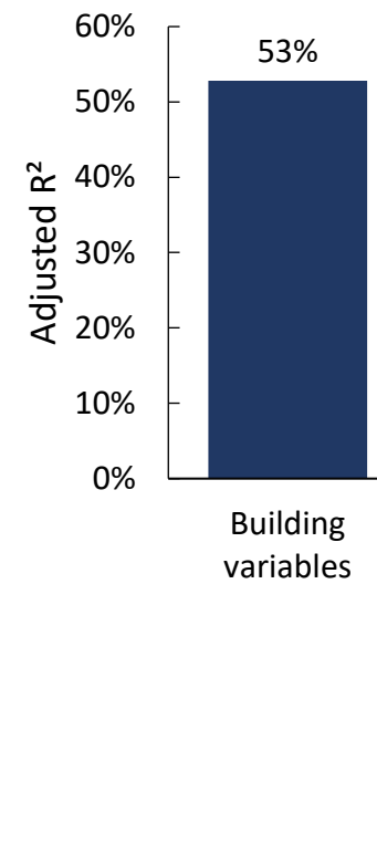
Explanatory power of combined LASSO regression models for SAP-predicted energy demand
