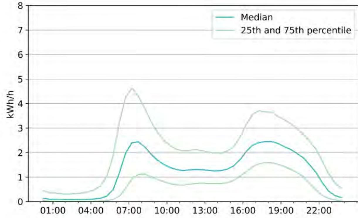
Average daily gas consumption
