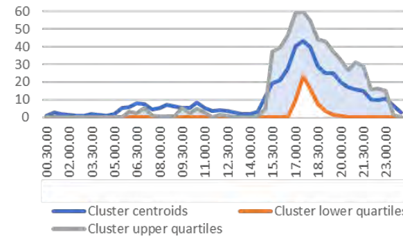
Nov-21, gas, cluster 8 (n=38)
