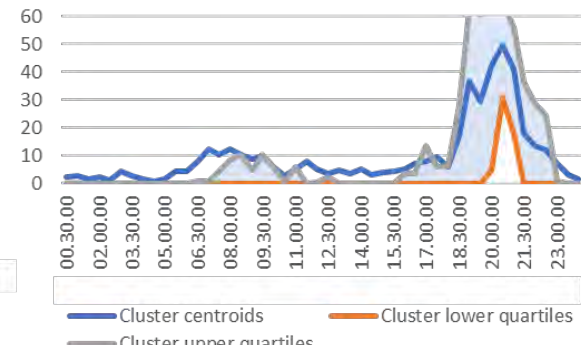
Nov-21, gas, cluster 9 (n=67)
