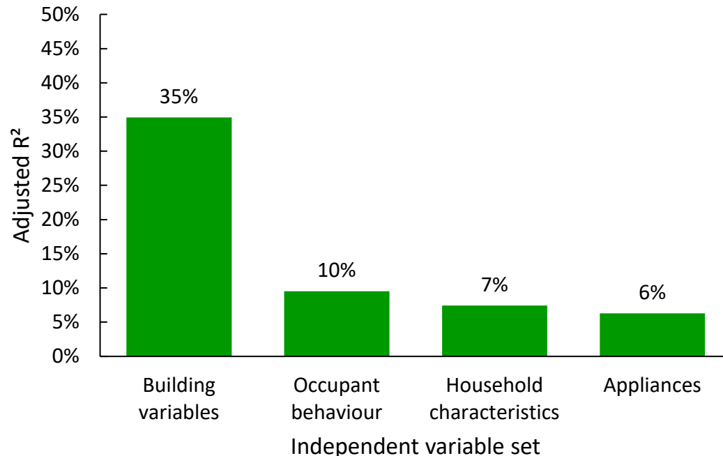
Explanatory power of individual LASSO regression models
